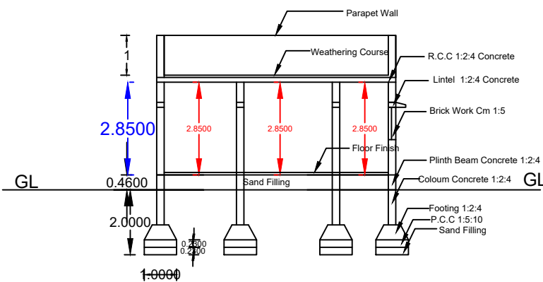
Section Section - AA
