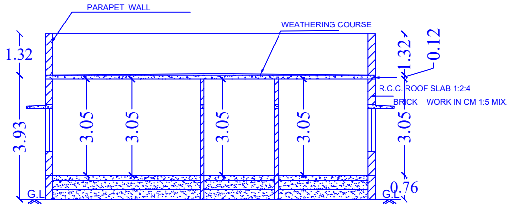
Section on-"AA"
