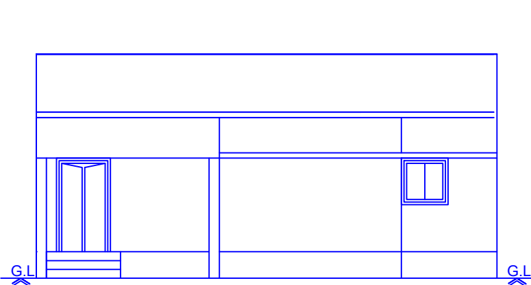
Front Elevation
