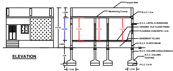
Section SECTION ON 'AA'
