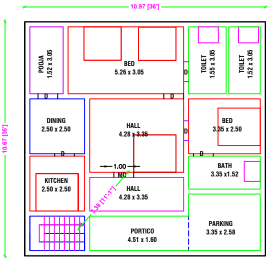
PRO.GROUND FLOOR PLAN EAST FACING
