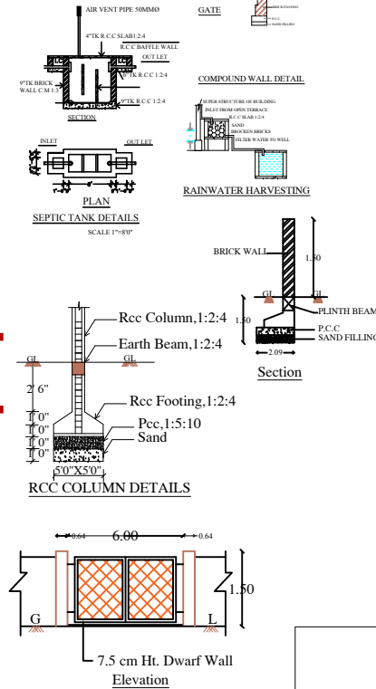
Section Details
