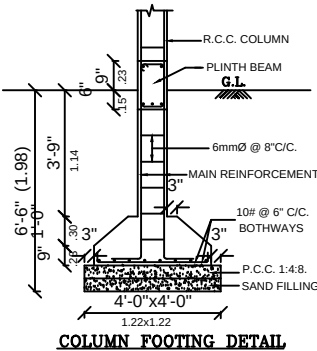
COLUMN FOOTING DETAIL
