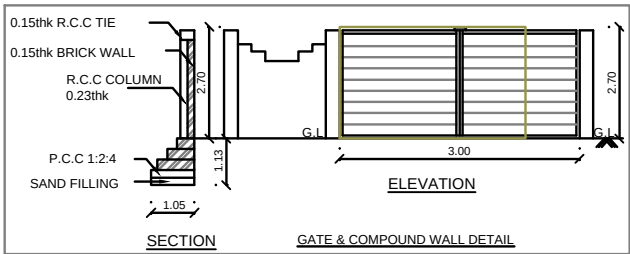
GATE & COMPOUND WALL DETAIL
