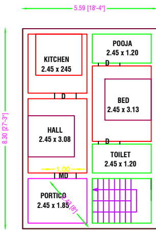
PRO. GROUND FLOOR PLAN [ NORTH FACING ]
