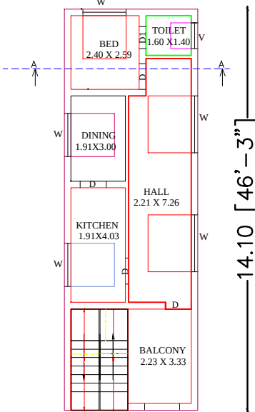
FIRST FLOOR PLAN (PROPOSED)
