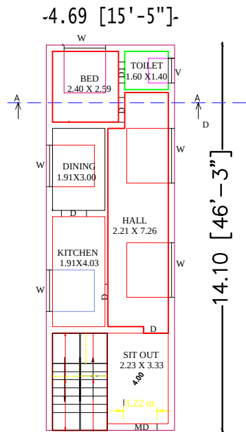
GROUND FLOOR PLAN (EXISTING)
