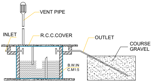
SEPTIC TANK & D-TRENCH DETAILS
