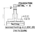
Foundation Detail - A (Not To Scale)
