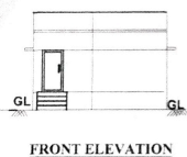
FRONT ELEVATION
