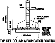
TYP. DET. COLUMN & FOUNDATION FOOTING
