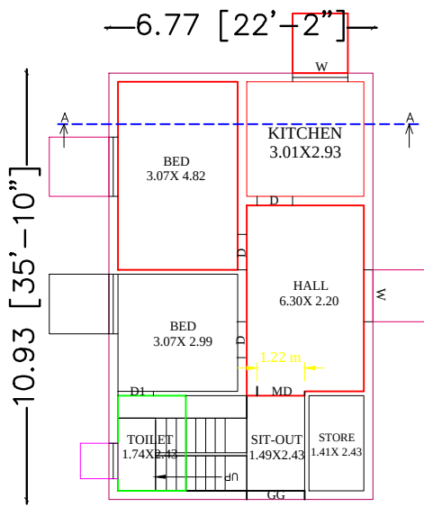
GROUND FLOOR PLAN RESIDENTIAL & COMMERCIAL (WEST FACING)
