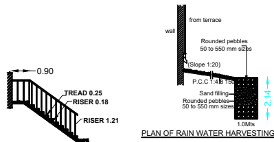
PLAN OF RAIN WATER HARVESTING
