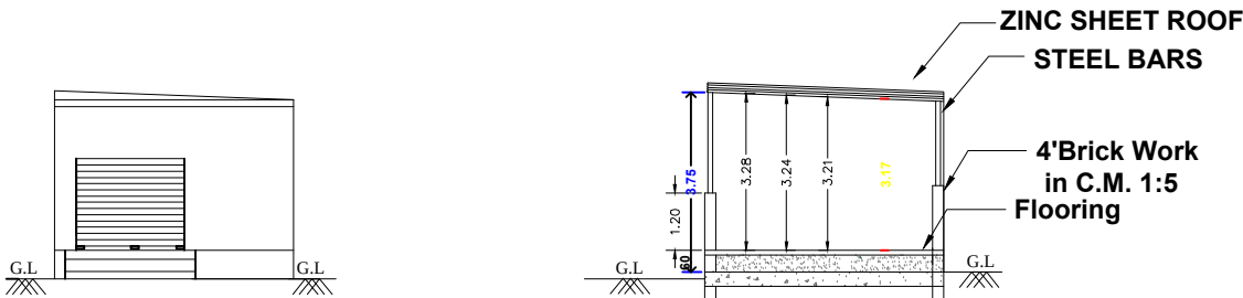
FRONT ELEVATION
