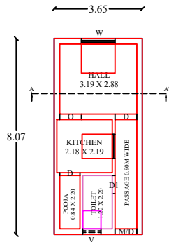
GROUND FLOOR PLAN (SOUTH FACING)
