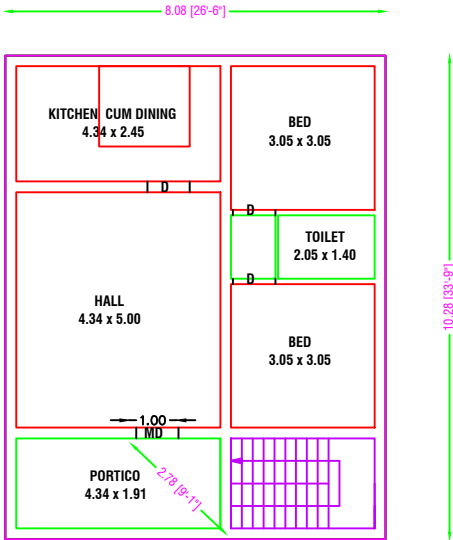
PRO. GROUND FLOOR PLAN [ NORTH FACING ]
