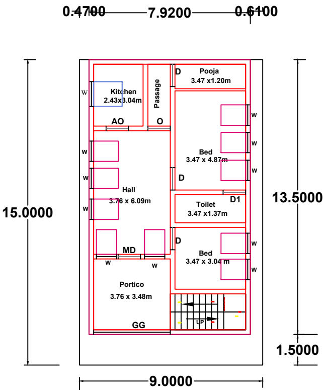
GROUND FLOOR PLAN ( NORTH FACING )
