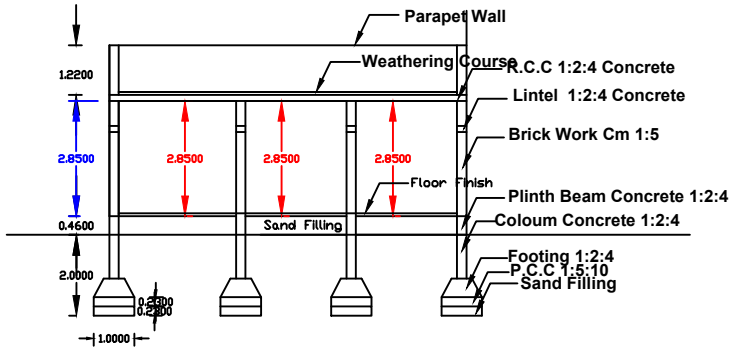
Section Section - AA
