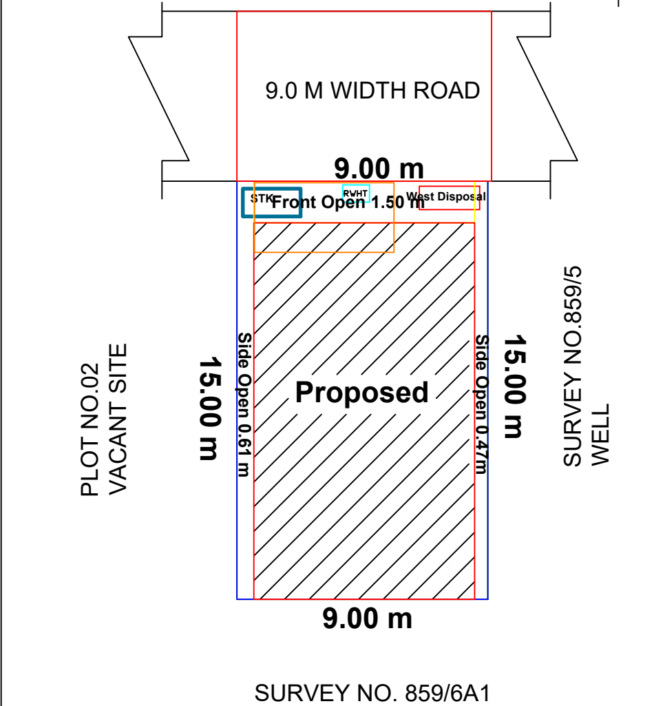
SITE PLAN
