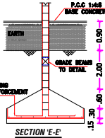
DETAILS OF COLUMN FOOTING
