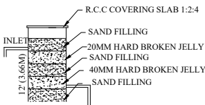
RAIN WATER HARVESTING
