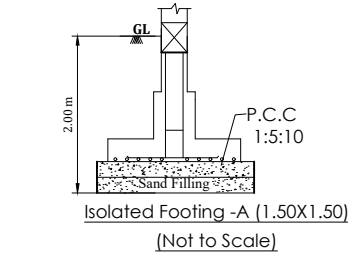
FOUNDATION DETAIL - A
