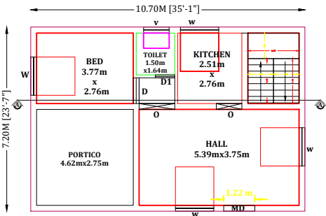
GROUND FLOOR PLAN (WEST FACING)
