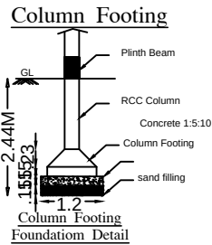
Column Footing Foundation Detail
