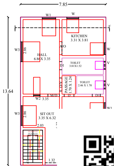
GROUND F (EAST)
