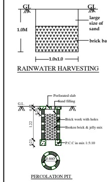
PERCOLATION PIT
