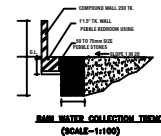
RAIN WATER COLLECTION ITEM (SCALE-1:100)
