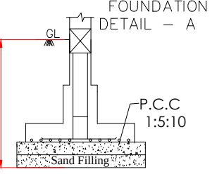
Isolated Footing -A (1.50X1.50) (Not to Scale)
