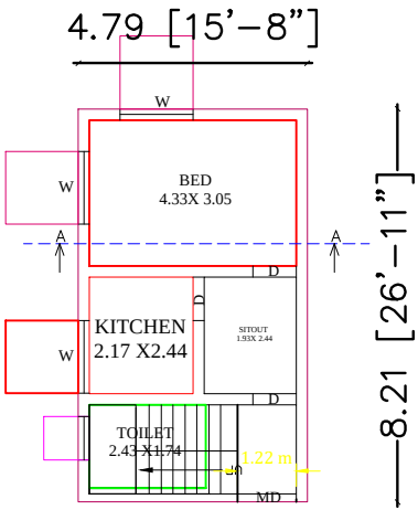
GROUND FLOOR PLAN (EAST FACING)
