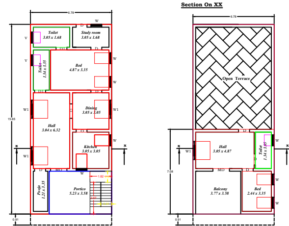
Exist Ground Floor Plan South facing
