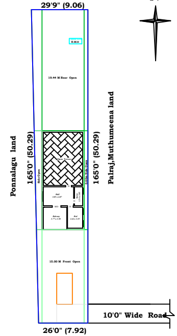
Thirumalai kumar house
