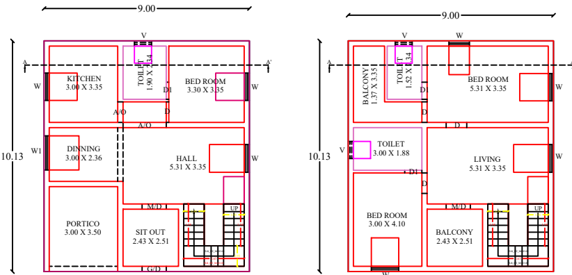
GROUND FLOOR PLAN (NORTH FACING)
