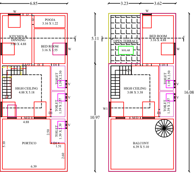
GROUND FLOOR PLAN (NORTH FACING)
