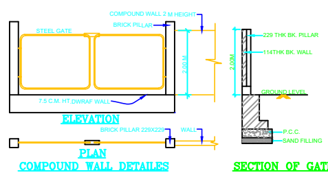
PLAN COMPOUND WALL DETAILS
