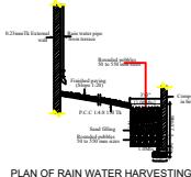
PLAN OF RAIN WATER HARVESTING
