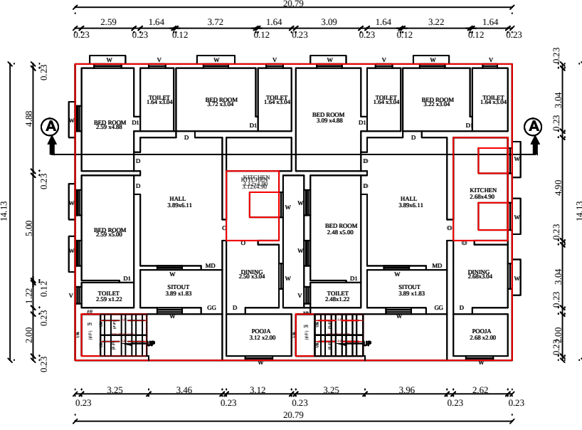
EXT.GROUND FLOOR PLAN
