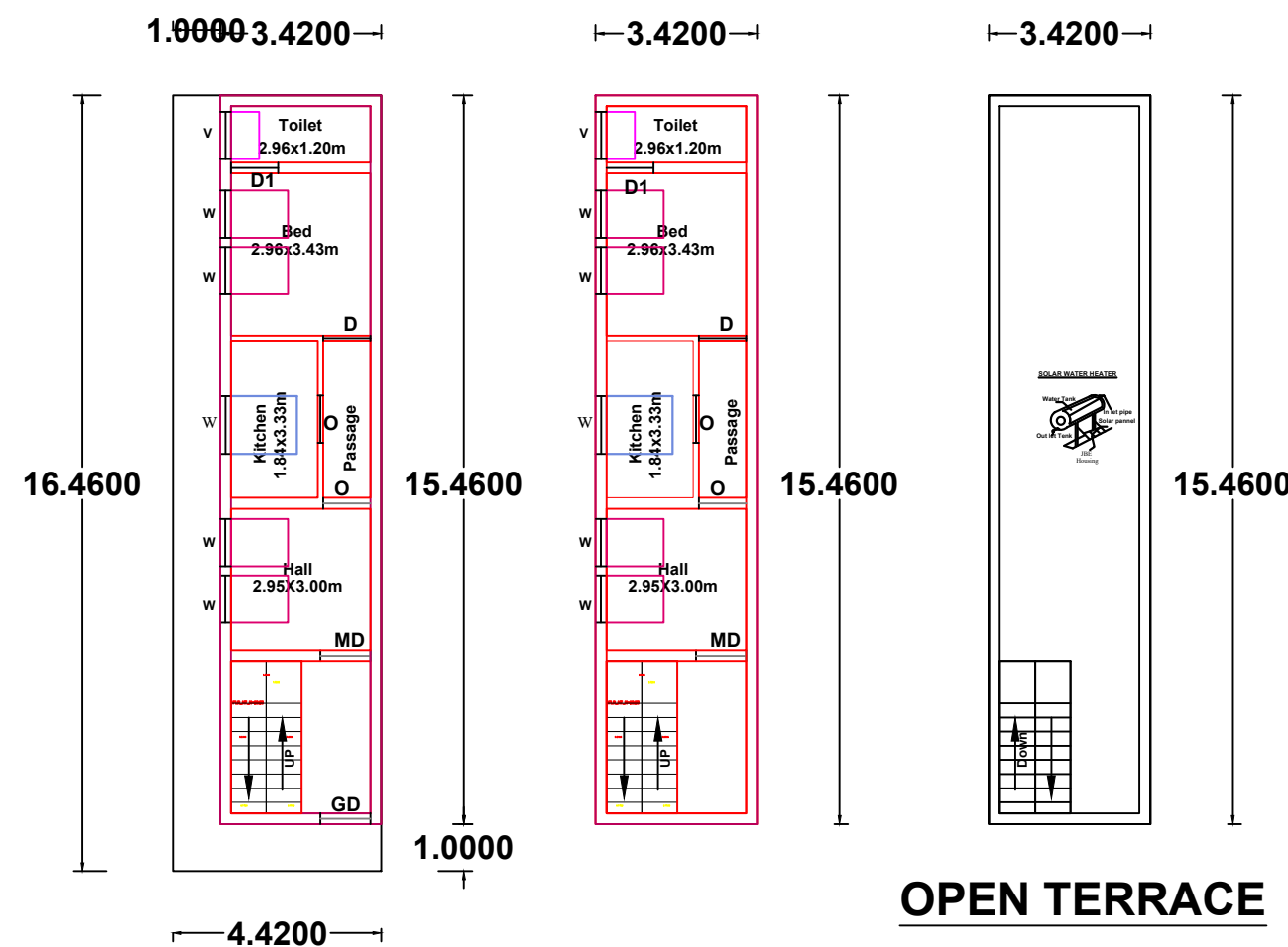
GROUND FLOOR
