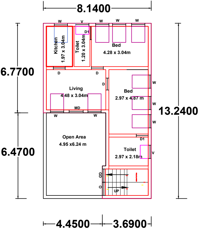
Proposed First Floor Floor
