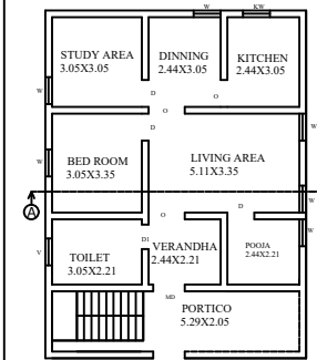
EXT.GROUND FLOOR PLAN
