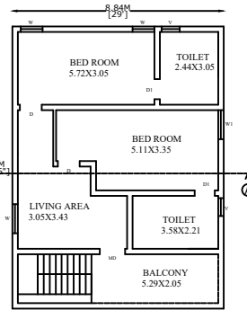
PROP.FIRST FLOOR PLAN
