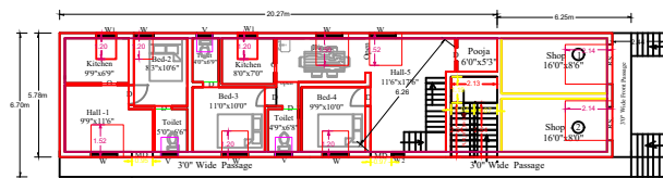
PROPOSED RESIDENTIAL & COMMERCIAL GROUND FLOOR PLAN
