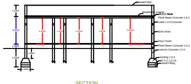
SECTION SECTION - AB
