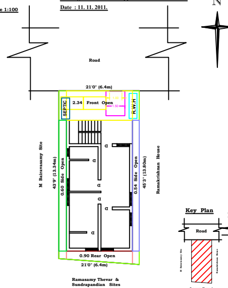
Site Plan
