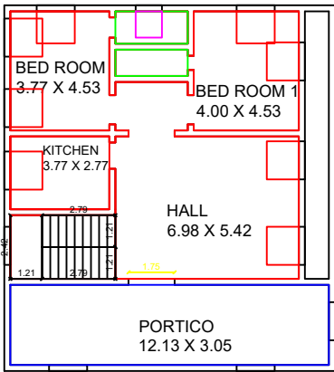
PROPOSED FIRST FLOOR AREA
