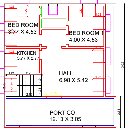
PROPOSED GROUND FLOOR AREA
