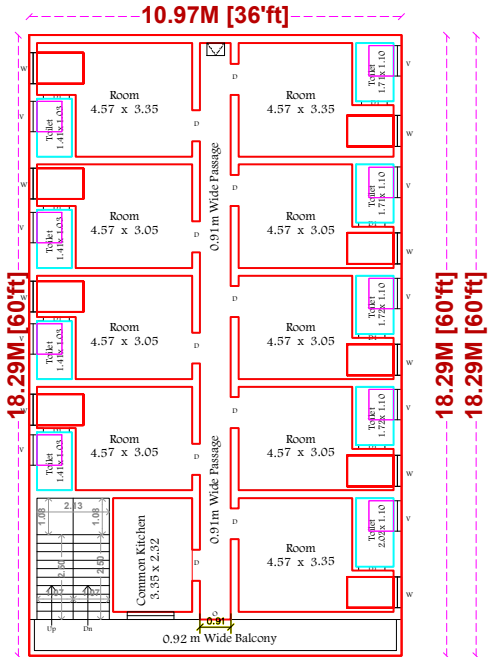
FIRST FLOOR RESIDENTIAL PLAN
