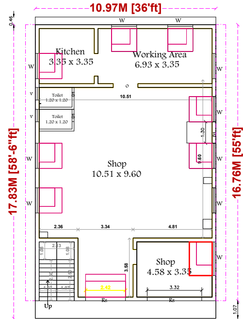
GROUND FLOOR COMMERCIAL PLAN
