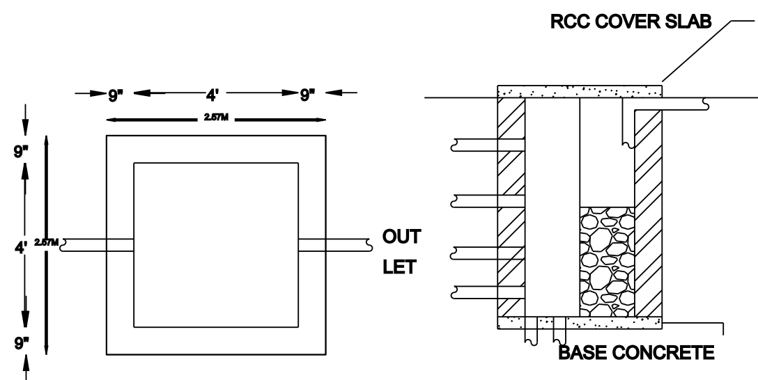
RAIN WATER COLLECTION PIT DETAILS
