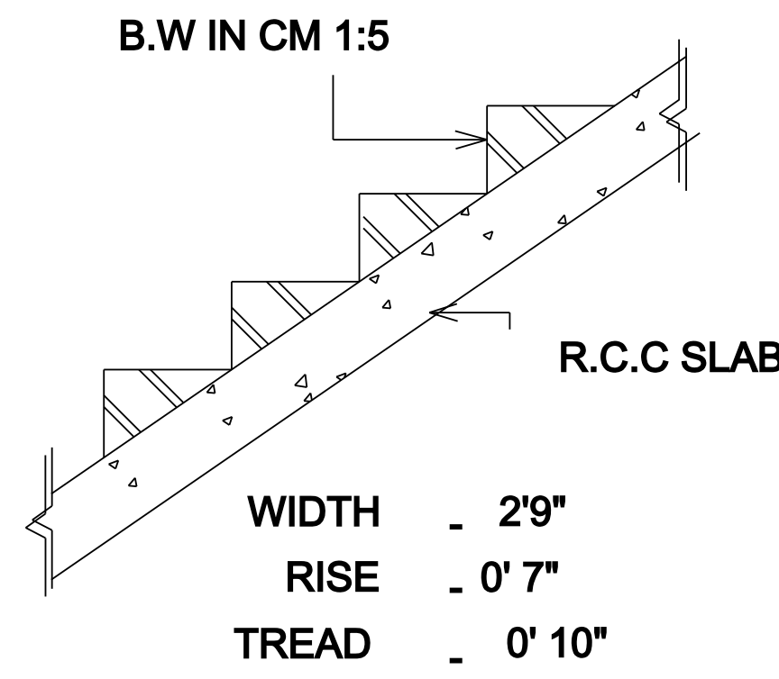
STAIR DETAILS
