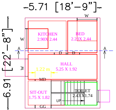
GROUND FLOOR PLAN (NORTH FACING)
