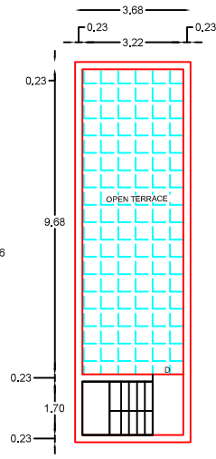
PROPOSED TERRACE FLOOR PLAN
