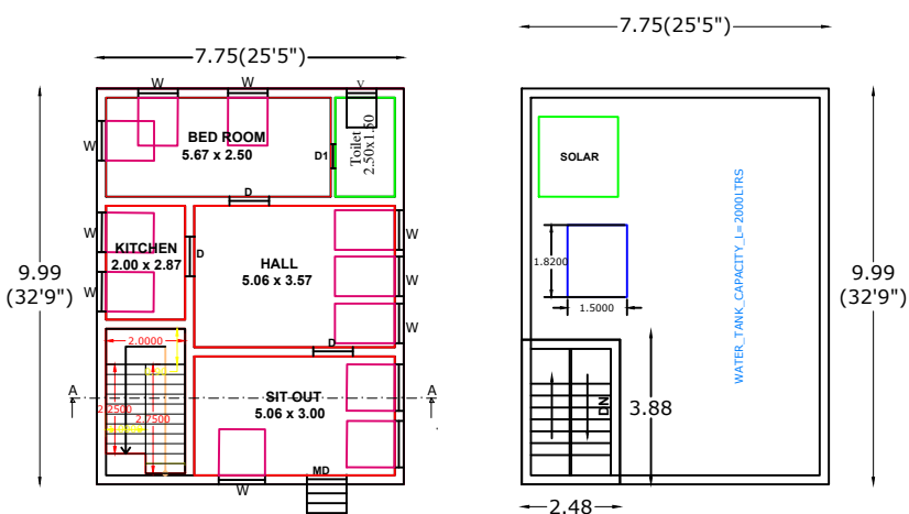
TERRACED FLOOR PLAN
