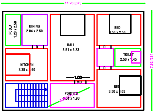
PRO.GROUND FLOOR PLAN EAST FACING
