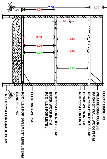
SECTION ON B-B'
