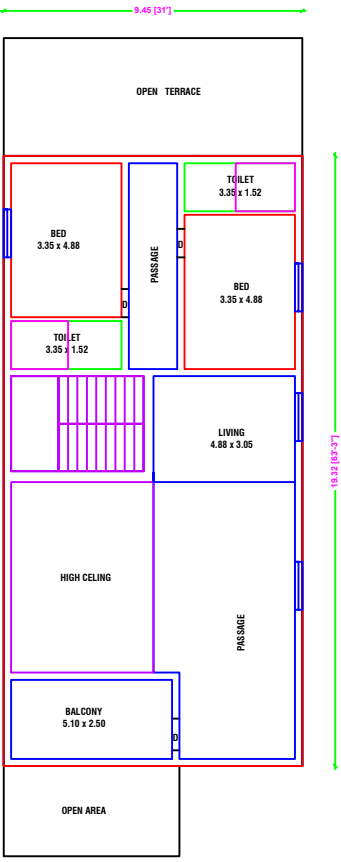
PRO.FIRST FLOOR PLAN WEST FACING
