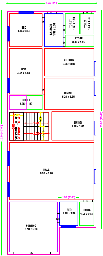
PRO.GROUND FLOOR PLAN WEST FACING
