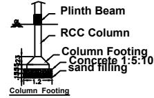
Foundation Detail
