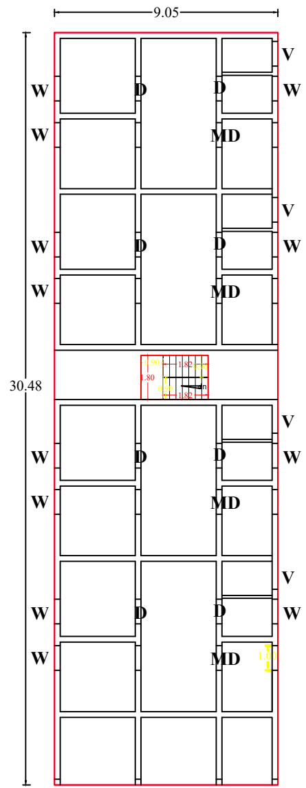
EXIS GROUND FLOOR PLAN
