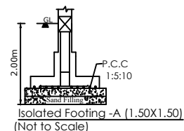
FOUNDATION DETAIL
