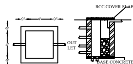
PLAN RAIN WATER COLLECTION PIT DETAILS
