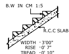
STAIR DETAILS
