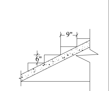
Staircase Detail Not To Scale
