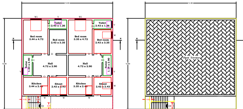
Proposed Terrace Floor Plan
