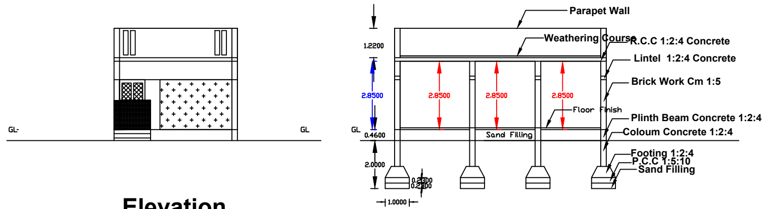
Section Section - AA
