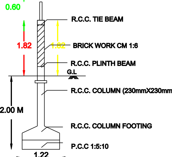
R.C.C. COLUMN FOOTING
